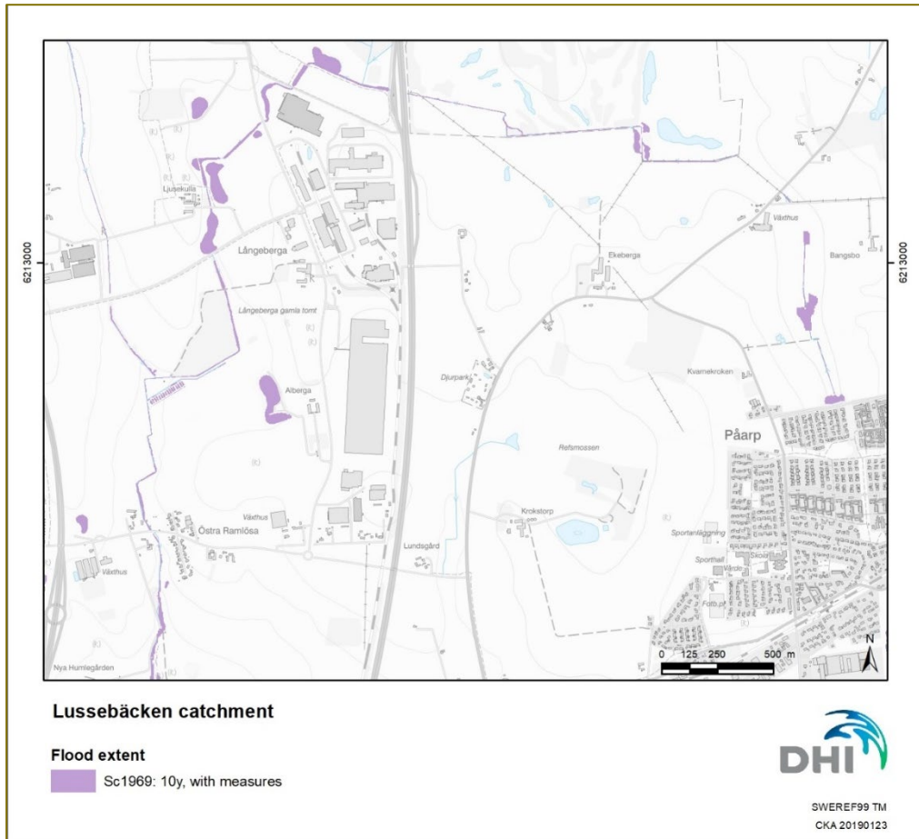
Figure 7 Calculated flood extent in the northern part of Lussebäcken for a 10-year flood event with measures and land use corresponding to the year 1969.
