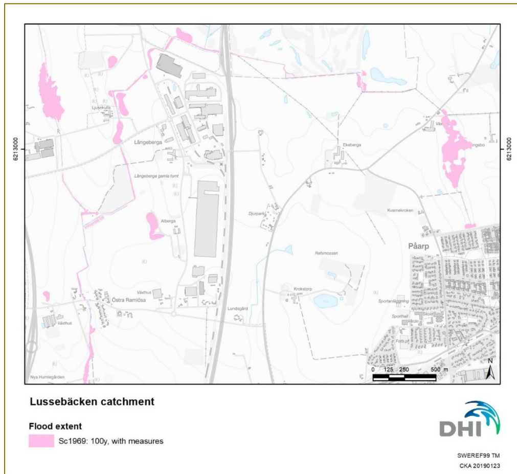
Figure 5 Calculated flood extent in the northern part of Lussebäcken for a climate adjusted 100-year flood event with measures and land use corresponding to the year 1969.
