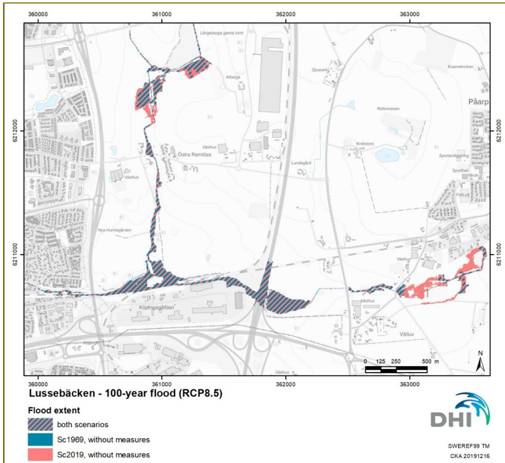
Figure 8 Calculated flood extent in the eastern part of Lussebäcken for a 100-year flood event where no water management measures have been conducted. Flood extent is presented for two scenarios of urbanization; 1969 and 2019.
