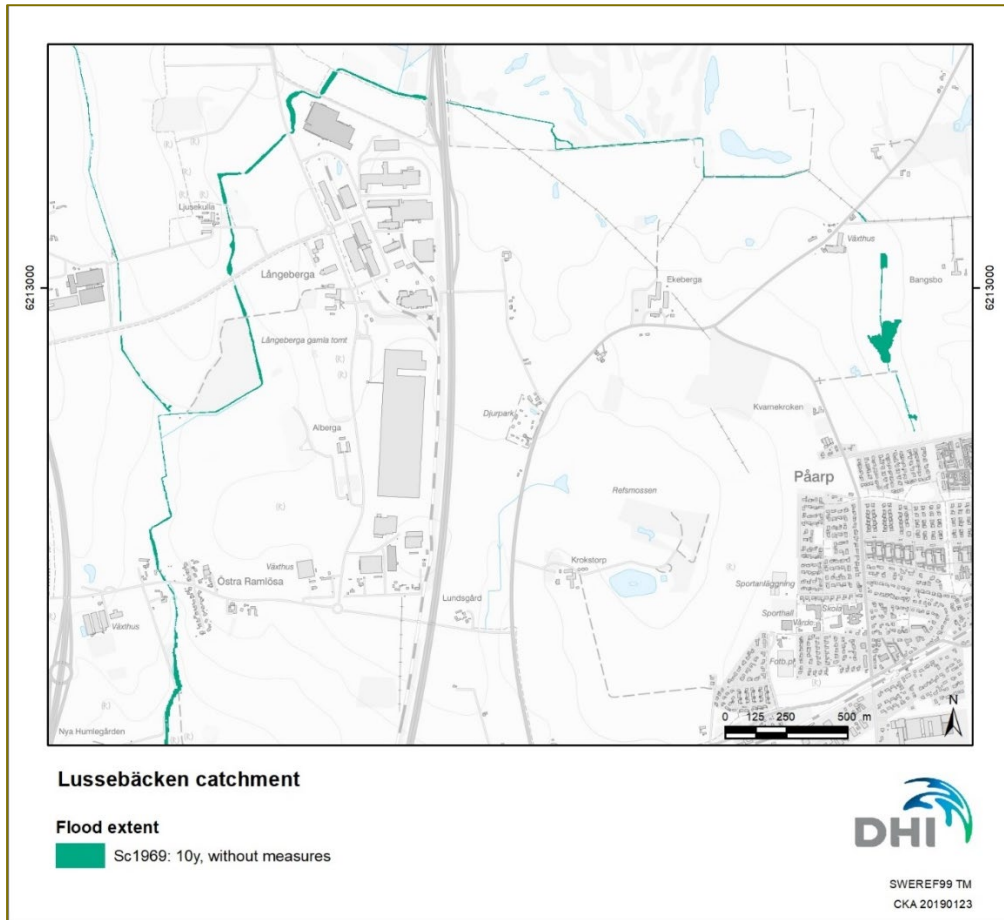
Figure 15 Calculated flood extent in the northern part of Lussebäcken for a 10-year flood event with no measures and land use corresponding to the year 1969.
