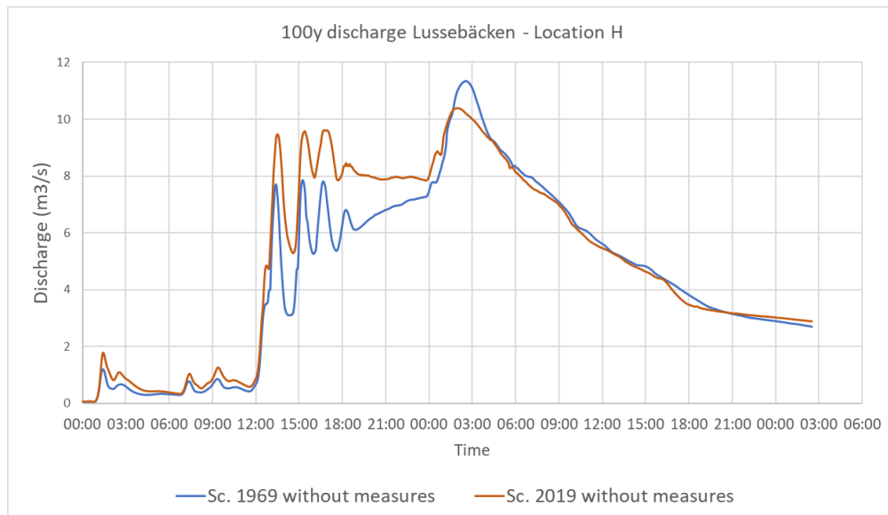
Figure 11 The 100-year discharge at location H. Presented are the scenarios without water management measures with land use of 1969 and 2019 respectively.
