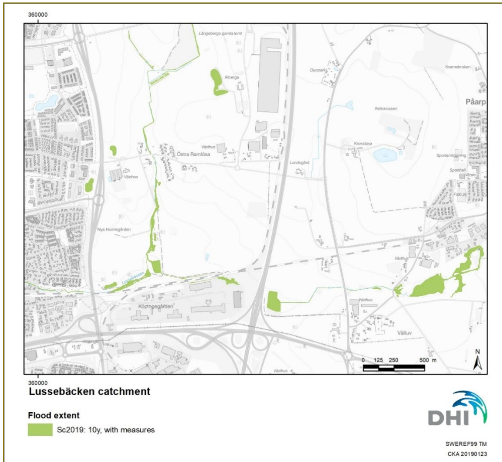
Figure 4 Calculated flood extent in the eastern part of Lussebäcken for a 10-year flood event with measures and land use corresponding to the year 2019.
