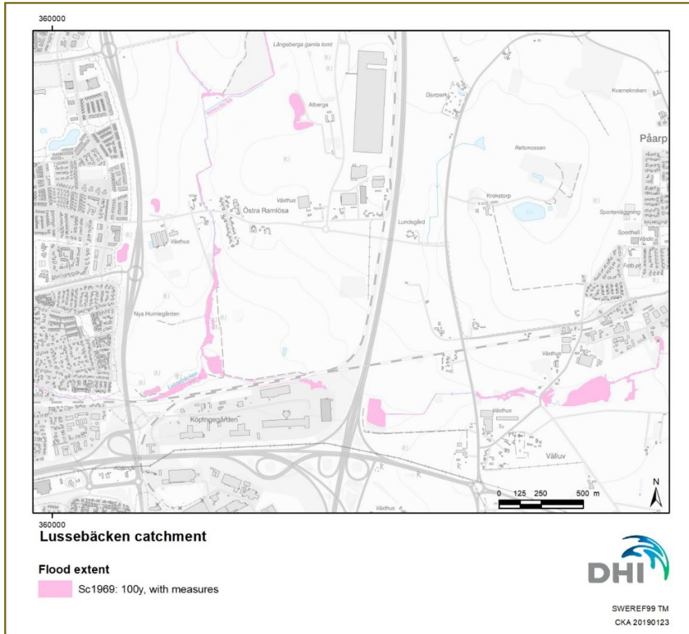
Figure 6 Calculated flood extent in the eastern part of Lussebäcken for a climate adjusted 100-year flood event with measures and land use corresponding to the year 1969.
