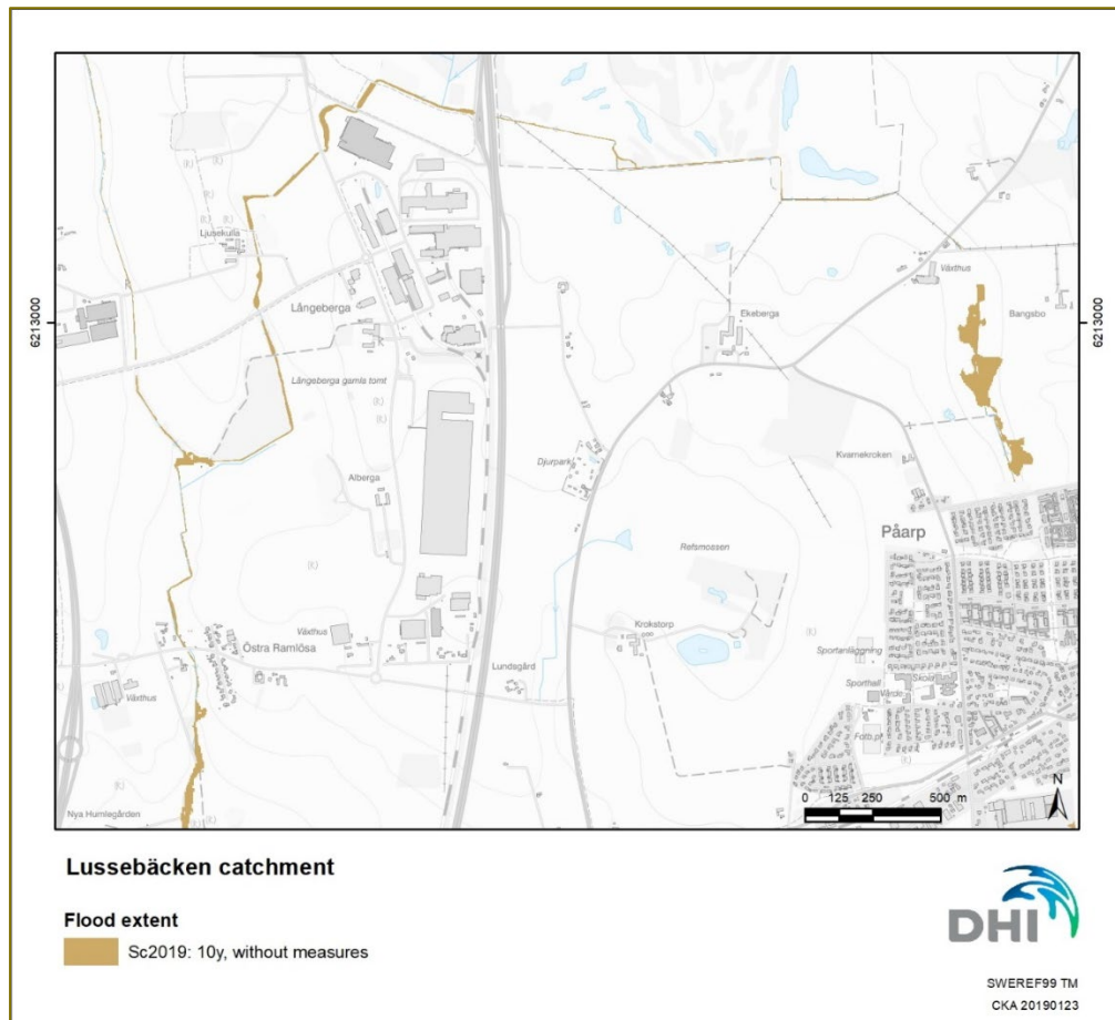
Figure 11 Calculated flood extent in the northern part of Lussebäcken for a 10-year flood event with no measures and land use corresponding to the year 2019.
