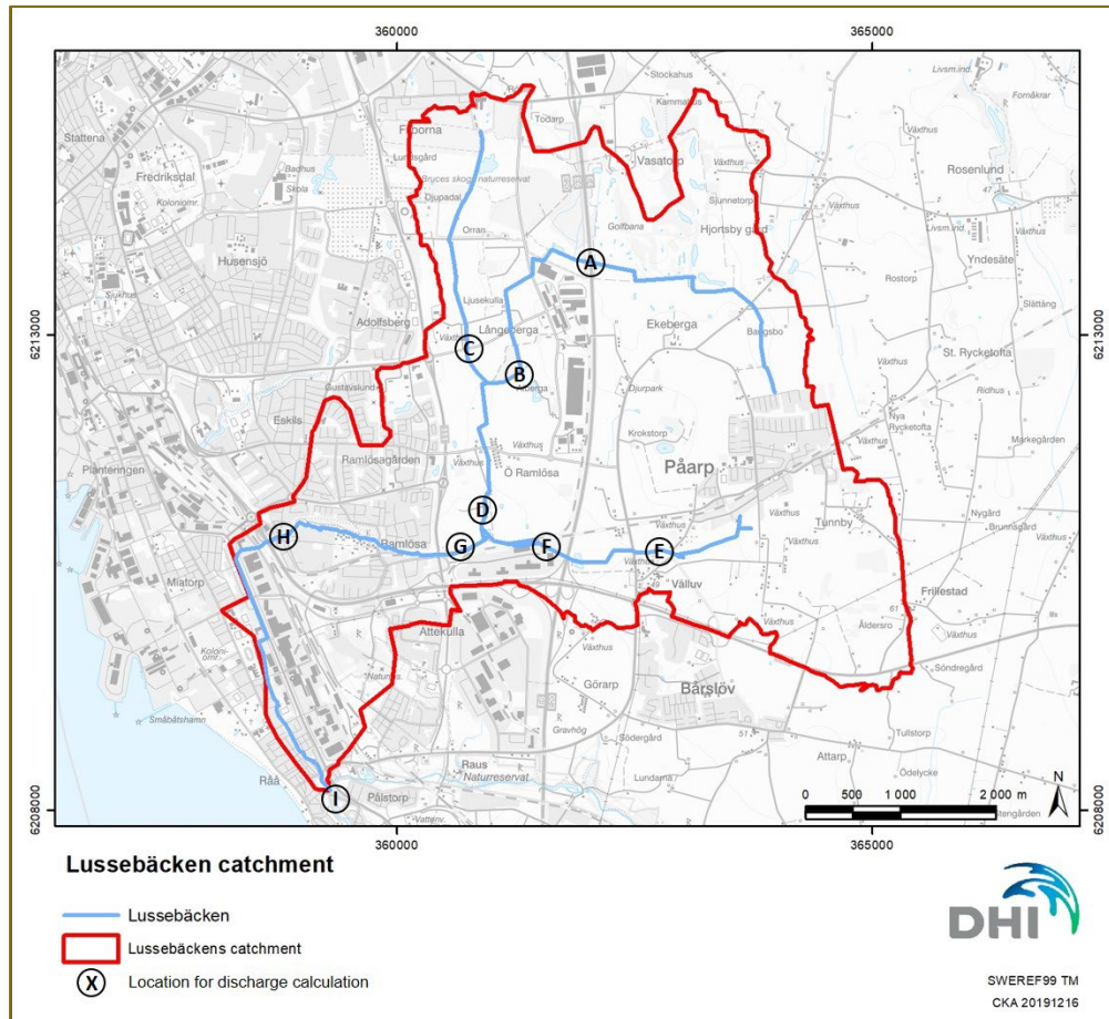
Figure 10 Locations along Lussebäcken where maximum discharge is calculated.
