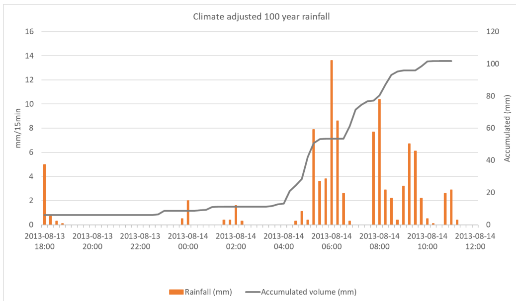
Figure 5 Climate adjusted 100 year rainfall, presented as load per 15 min together with accumulated rain volume.
