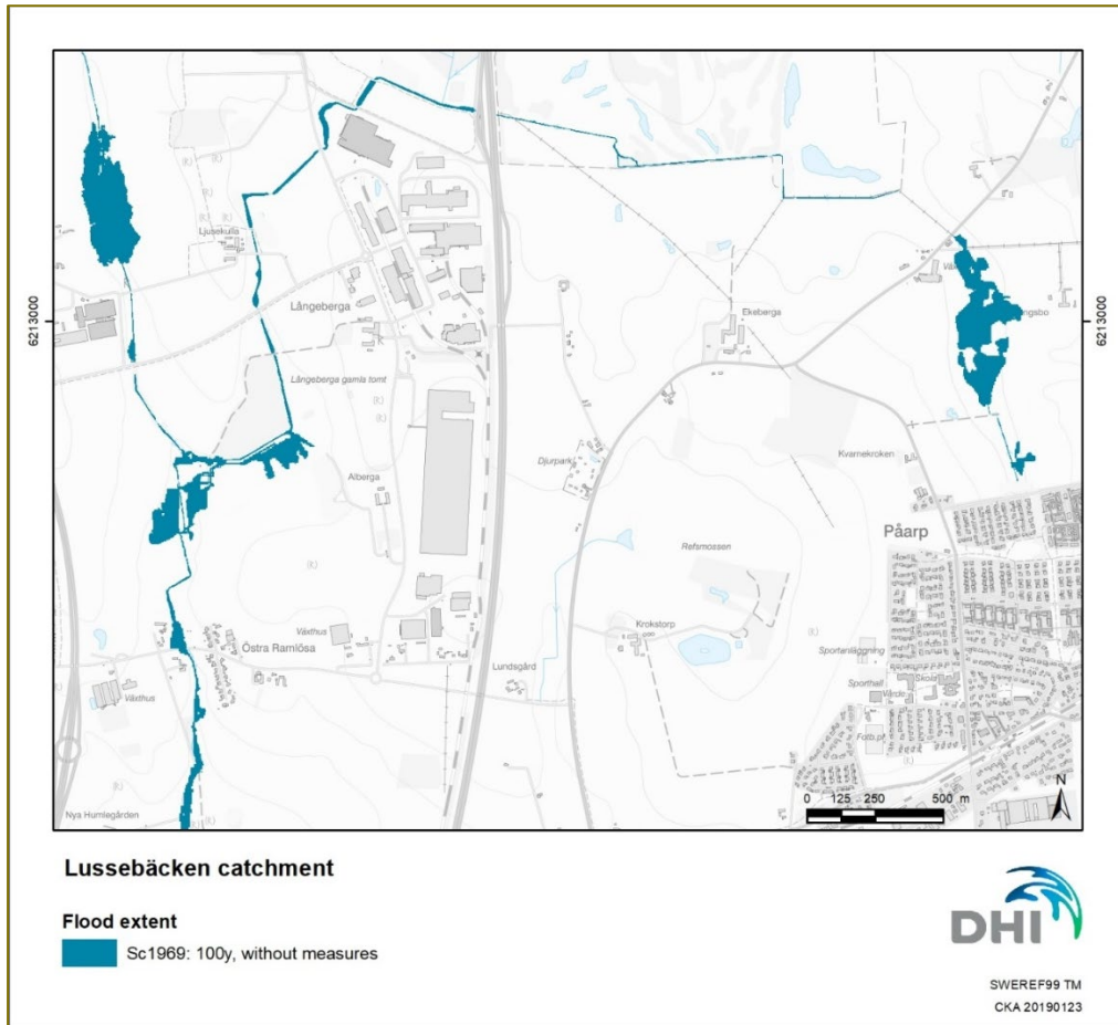
Figure 13 Calculated flood extent in the northern part of Lussebäcken for a climate adjusted 100-year flood event with no measures and land use corresponding to the year 1969.
