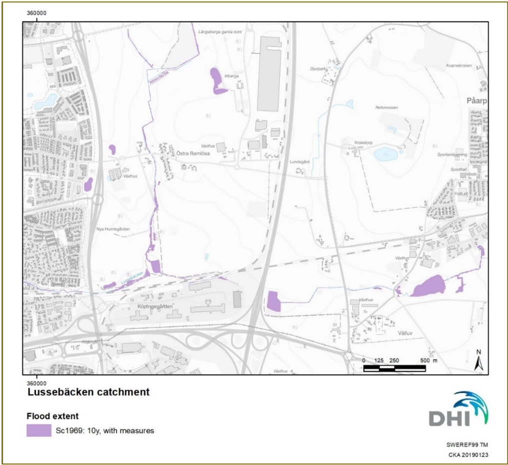
Figure 8 Calculated flood extent in the eastern part of Lussebäcken for a 10-year flood event with measures and land use corresponding to the year 1969.
