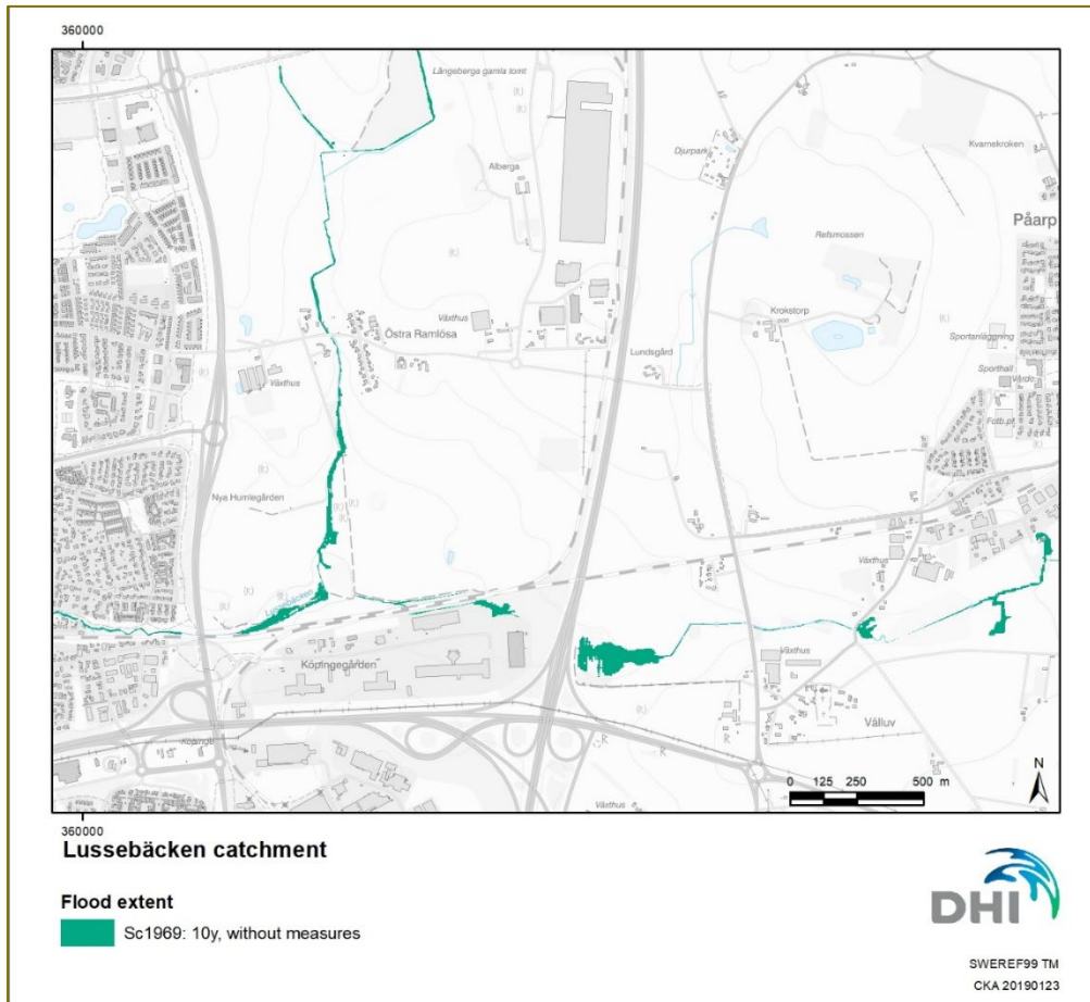
Figure 16 Calculated flood extent in the eastern part of Lussebäcken for a 10-year flood event with no measures and land use corresponding to the year 1969.
