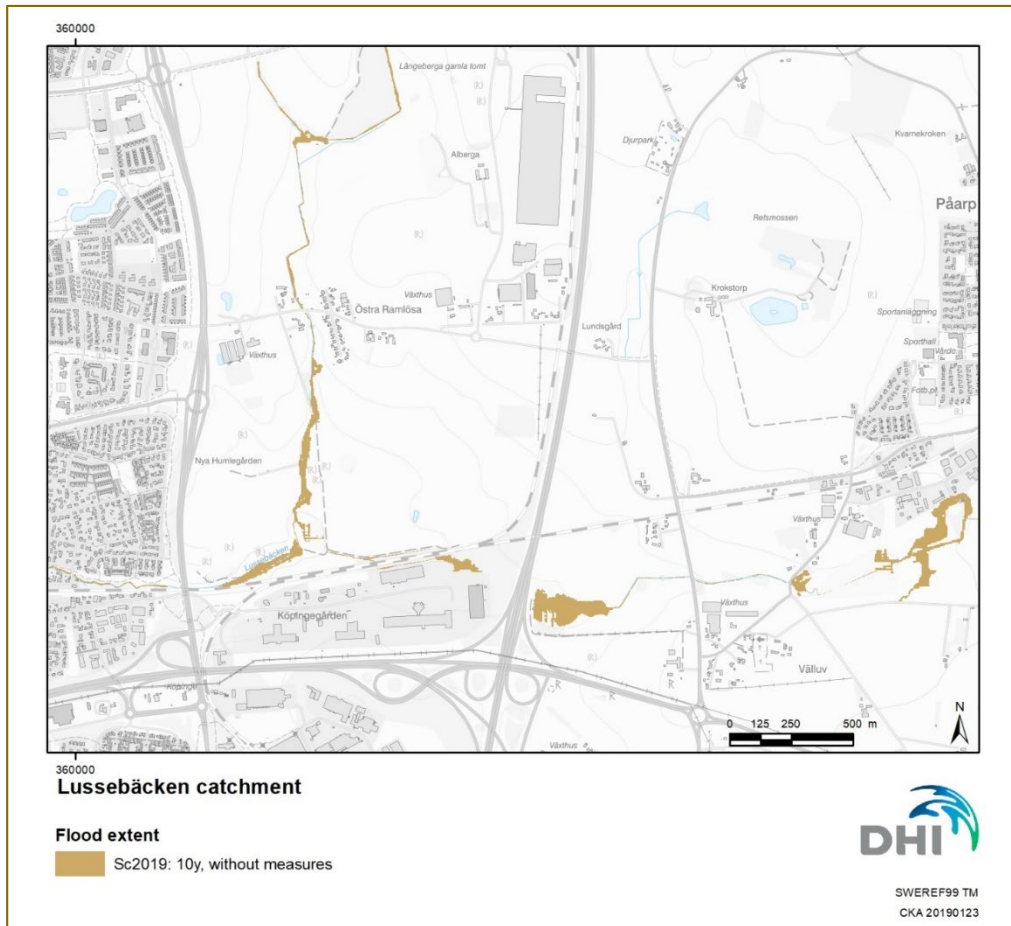
Figure 12 Calculated flood extent in the eastern part of Lussebäcken for a 10-year flood event with no measures and land use corresponding to the year 2019.
