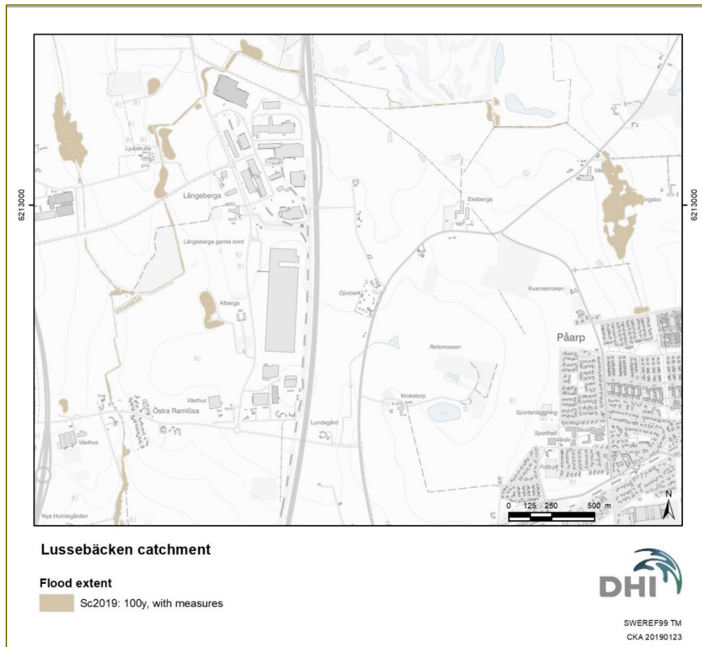
Figure 1 Calculated flood extent in the northern part of Lussebäcken for a climate adjusted 100-year flood event with measures and land use corresponding to the year 2019.
