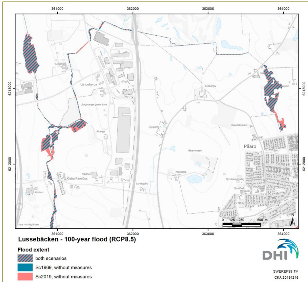
Figure 9 Calculated flood extent in the northern part of Lussebäcken for a 100-year flood event where no water management measures have been conducted. Flood extent is presented for two scenarios of urbanization; 1969 and 2019.
