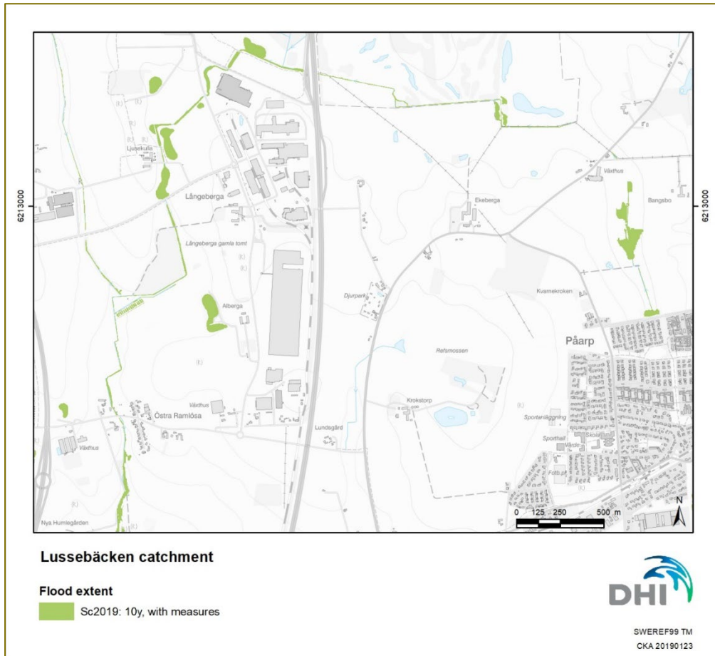
Figure 3 Calculated flood extent in the northern part of Lussebäcken for a 10-year flood event with measures and land use corresponding to the year 2019.
