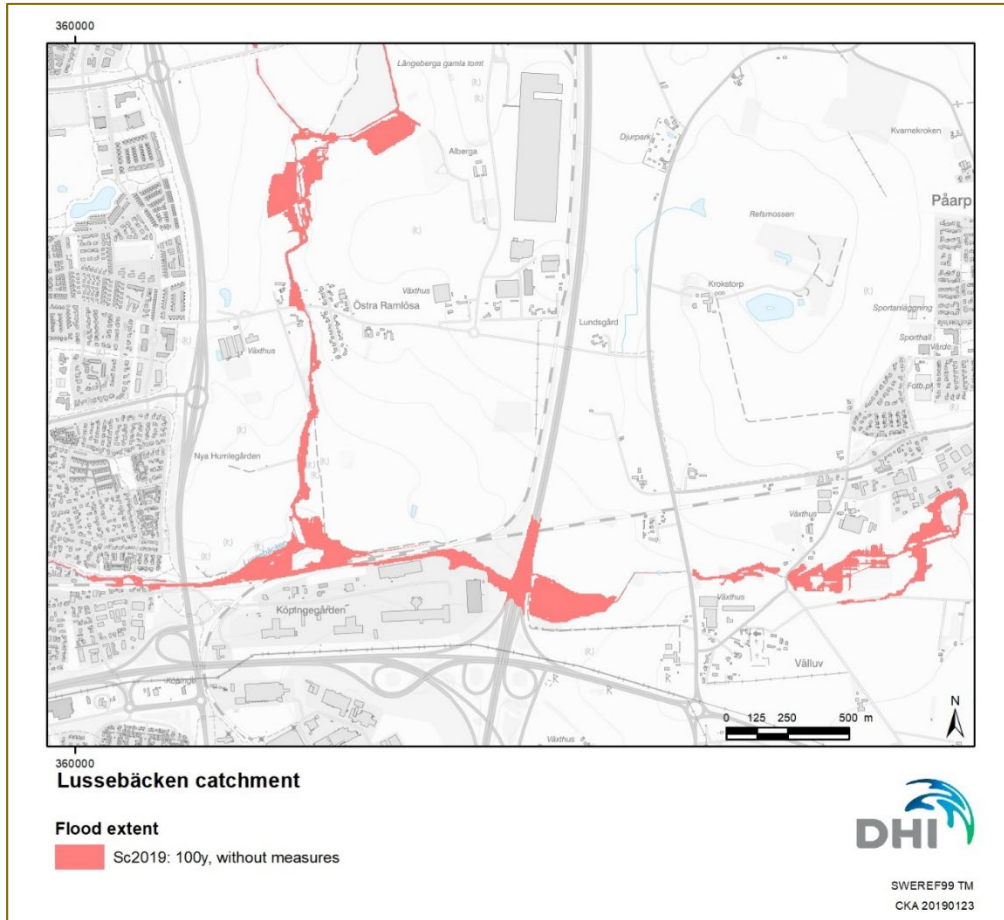
Figure 10 Calculated flood extent in the eastern part of Lussebäcken for a climate adjusted 100-year flood event with no measures and land use corresponding to the year 2019.
