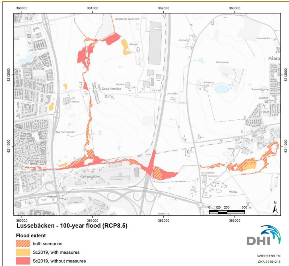
Figure 7 Calculated flood extent in the eastern part of Lussebäcken for a 100-year flood event with land use corresponding to the year 2019. Flood extent is presented for two scenarios with and without measures.
