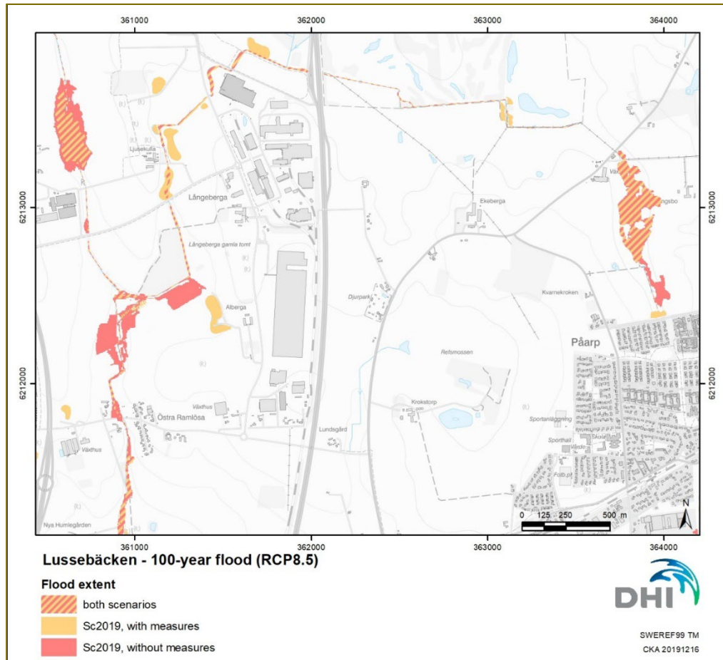
Figure 6 Calculated flood extent in the northern part of Lussebäcken for a 100-year flood event with land use corresponding to the year 2019. Flood extent is presented for two scenarios with and without measures.
