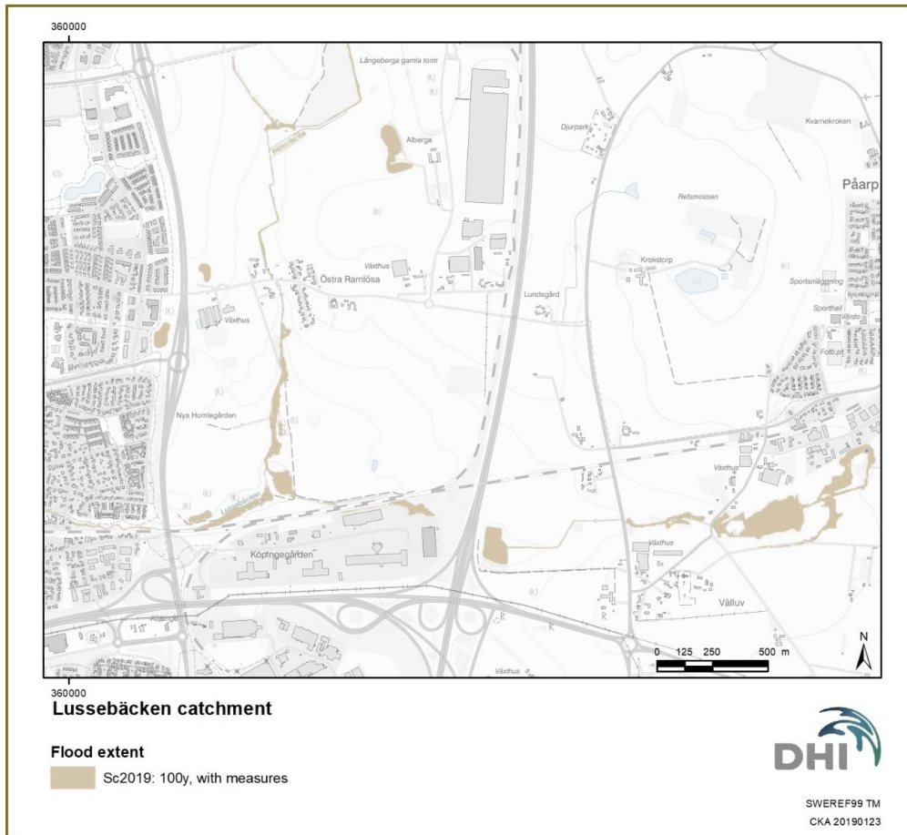
Figure 2 Calculated flood extent in the eastern part of Lussebäcken for a climate adjusted 100-year flood event with measures and land use corresponding to the year 2019.
