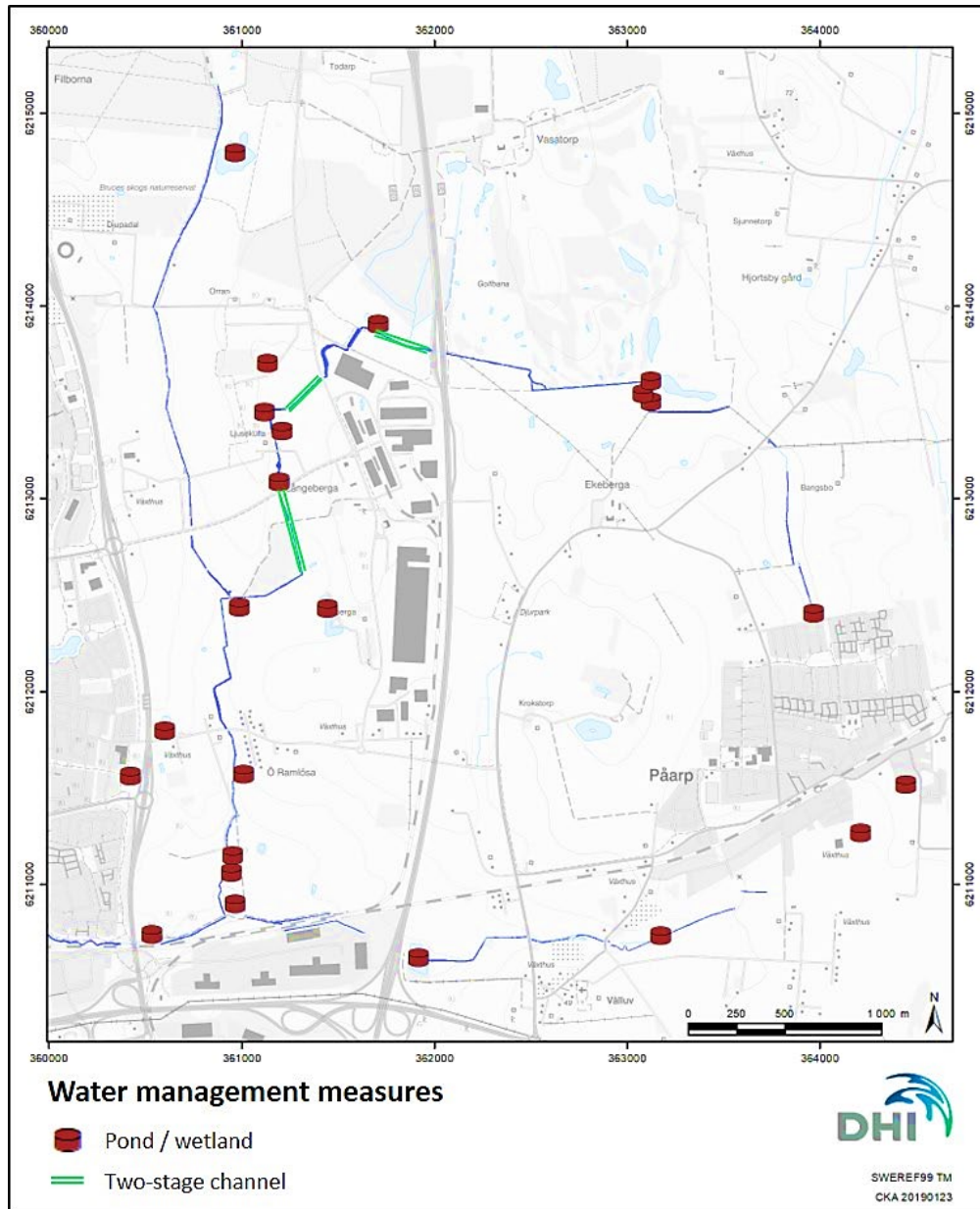
Figure 1 Water management measures in Lussebäcken catchment.
