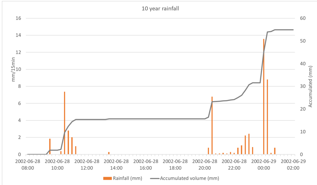
Figure 4 10 year rainfall, presented as load per 15 min together with accumulated rain volume.
