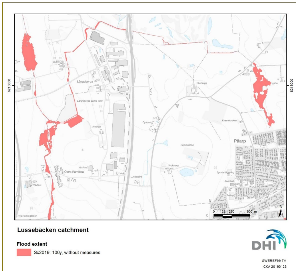
Figure 9 Calculated flood extent in the northern part of Lussebäcken for a climate adjusted 100-year flood event with no measures and land use corresponding to the year 2019.
