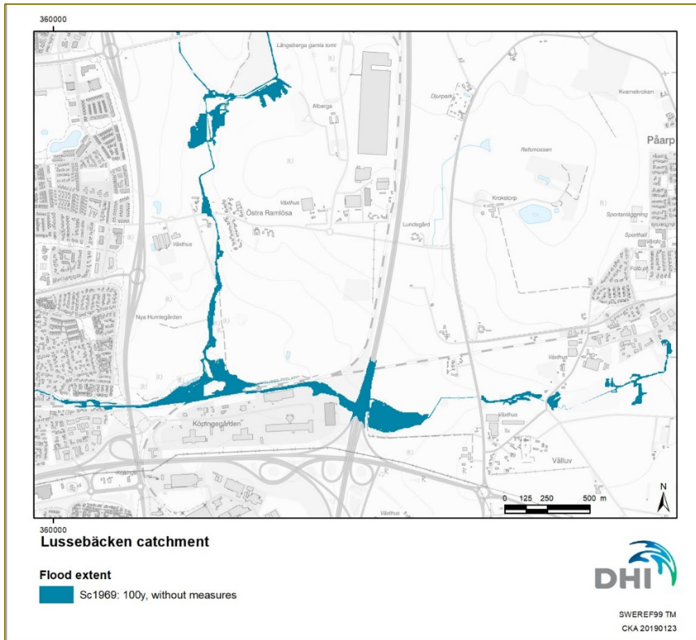
Figure 14 Calculated flood extent in the eastern part of Lussebäcken for a climate adjusted 100-year flood event with no measures and land use corresponding to the year 1969.
