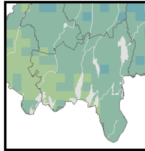
Observerat 1991-2013
