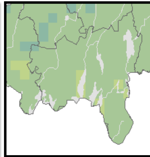
Observerat 1991-2013
