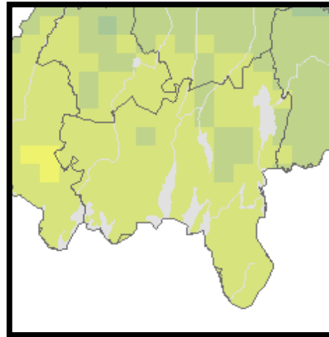
Observerat 1991-2013
