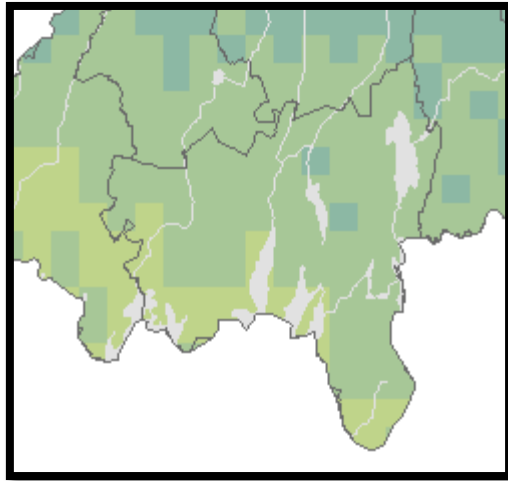
Observerat 1961-1990
