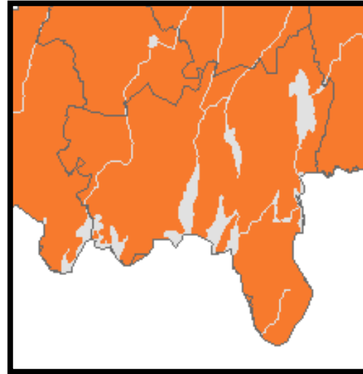
Observerat 1991-2013
