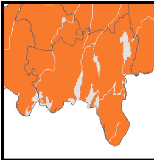
Observerat 1961-1990
