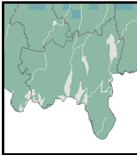
Observerat 1961-1990
