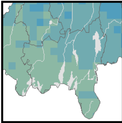
Observerat 1961-1990
